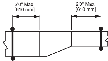
Figure 6-6 OFFSET REDUCER
